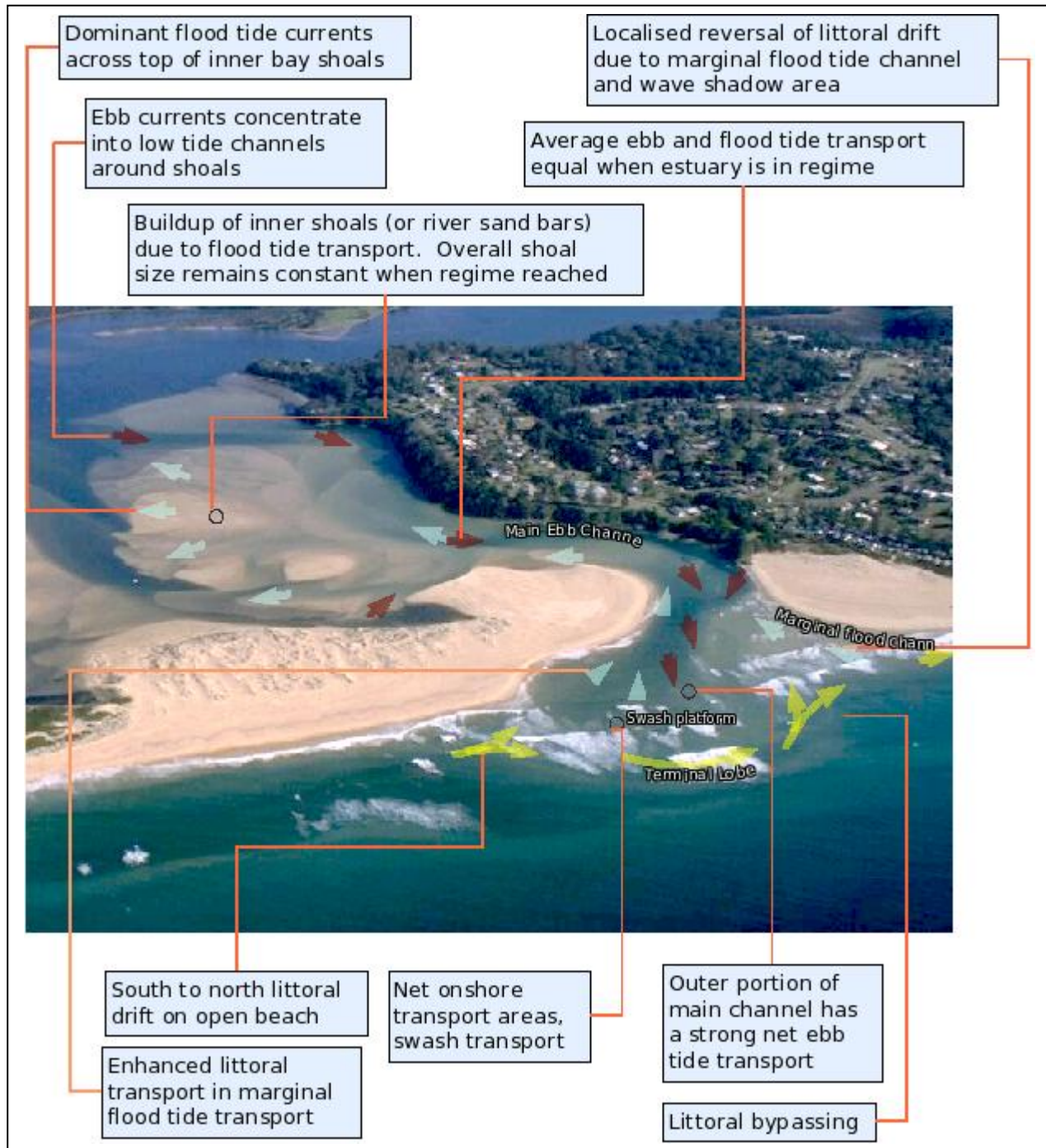
Figure 26 Sediment Pathways at a heavily shoaled entrance
